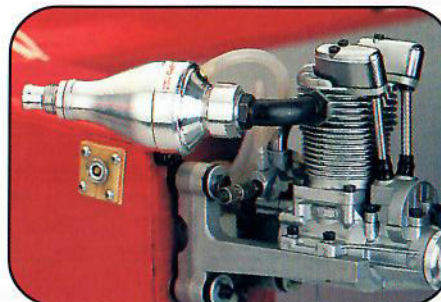
4-Stroke Muffler designed to fit most .40 to 1.50 engines with correct adapter.
